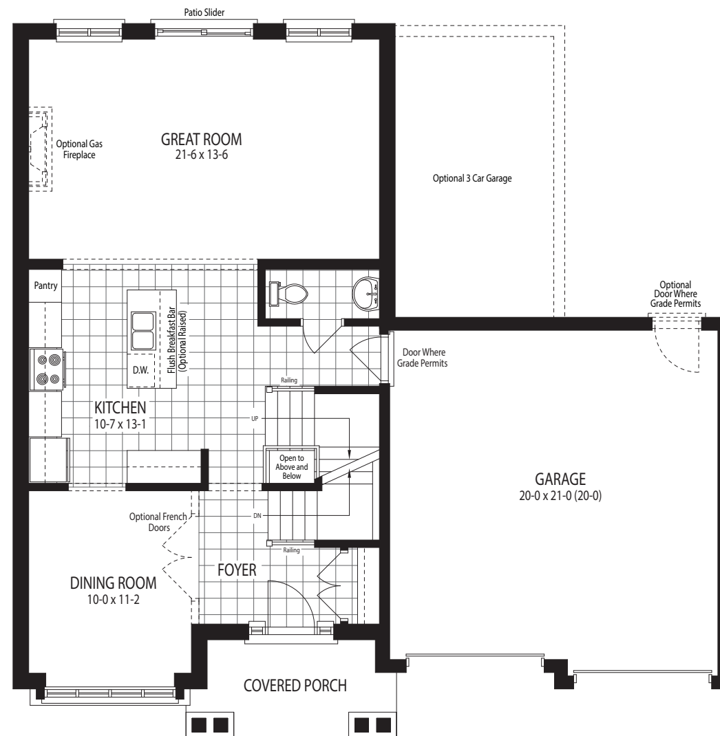
Main Floor
